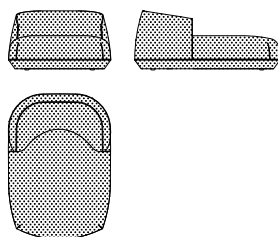
Daybed L 109 P 154 H 62 cm W 42 \frac{7}{8} " D 60 \frac{5}{8} " H 24 \frac{3}{8} "
