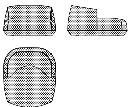
Lounge armchair large L 109 P 124 H 62 cm W 42 \frac{7}{8} " D 48 \frac{7}{8} " H 24 \frac{3}{8} "
